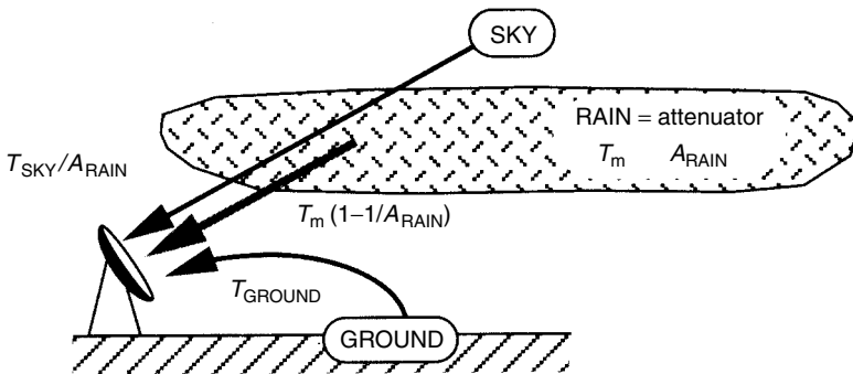
Figure 5.21 Components of earth station antenna noise temperature for rain conditions
