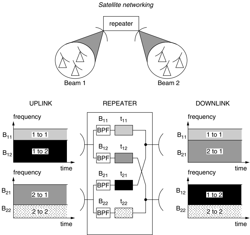
Figure 2.9 Interconnectivity of beams by permanent connections. (Reproduced from (MAR02) by permission of John Wiley & Sons Ltd) BPF: band pass filter. t_{ij} : transponder connecting beam i to beam j and operating in band B_{ij}
